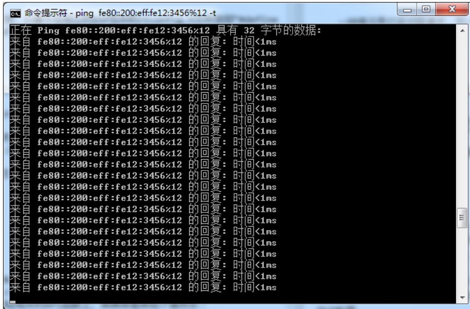
图 16.4: Link-local Address
